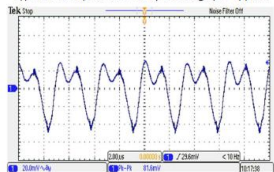
Figure 8 : Output Voltage Ripple & Noise at full load. ( V_{in} : Typical, With Output Capacitor to add 10 \mu\text{F} MLCC)
