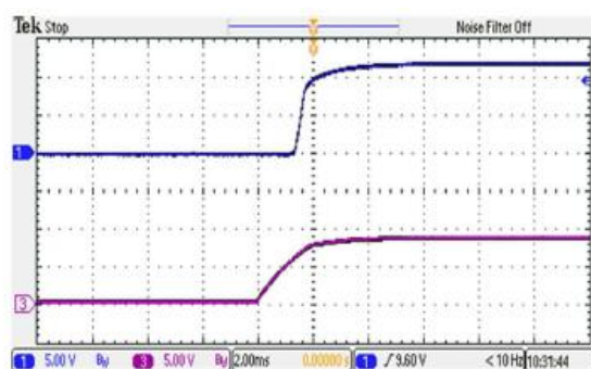
Figure 6 : CH1 = Vout, CH3 = Enable Pin Typical Start-up waveform. Input voltage pre-applied
