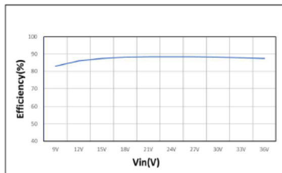
Figure 2 : Efficiency VS. Input Voltages at 100% rated power
